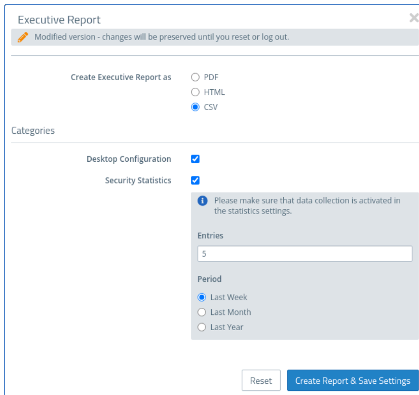
Figure 19: Executive Report – settings
