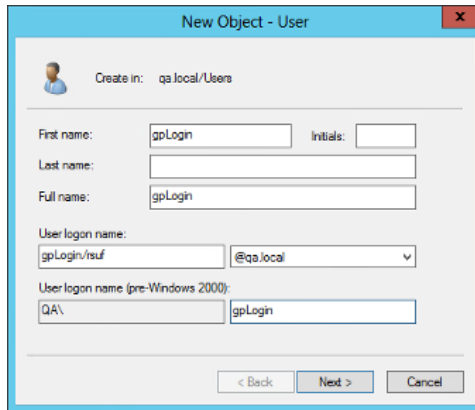
Figure 35: Create a user
